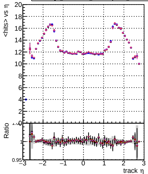
mean hits vs \eta DOM originals DOM testMKFit initialStepReso DOM testMKFit initialStepReso test100 DOM testMKFit initialStepReso test100bf
