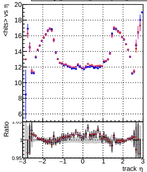
DOM originals DOM testMkFit initialStepReso DOM testMkFit initialStepReso test100 DOM testMkFit initialStepReso test100bf mean hits
