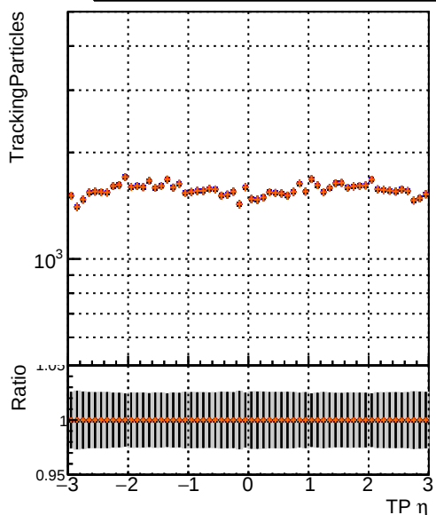
● DQM_original4 ● DQM_testMkFit_initialStepReso ● DQM_testMkFitFit_initialStepReso ● DQM_testMkFitFit_initialStepReso_Chi2Zero
