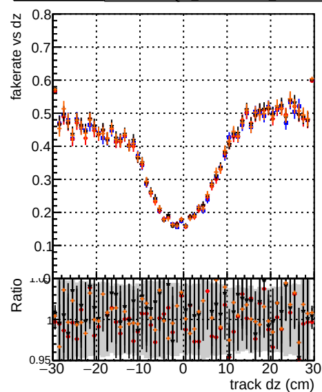
Fake rate vs dz Chi2Zero
