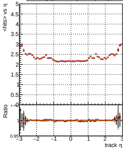
— DQM_original4 — DQM_testMkFit_initialStepReso — DQM_testMkFitFit_initialStepReso — DQM_testMkFitFit_initialStepReso_Chi2Zero
