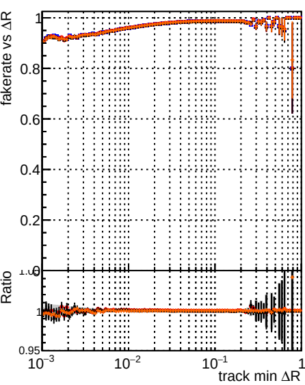
Fake rate vs \Delta R(\text{track, jet}) original4 testIMKFit_initialStepReso testIMKFit_initialStepReso_chi2Zero
