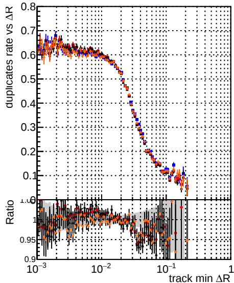
DOM original4 DOM testMKFit initialStepReso DOM testMKFit initialStepReso DOM testMKFit initialStepReso Chi2Zero
