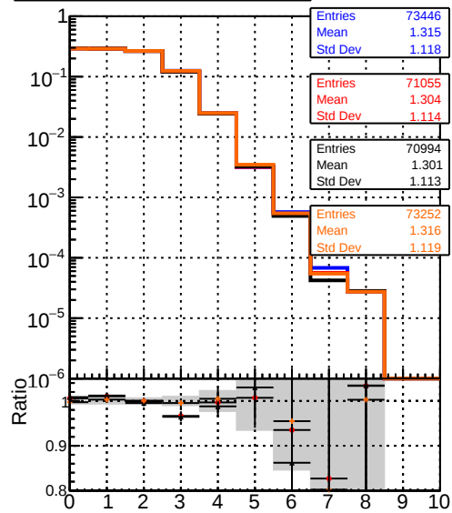
DQM_original4 DQM_testMkFit_initialStepReso DQM_testMkFitFit_initialStepReso DQM_testMkFitFit_initialStepReso_Chi2Zero mean hits
