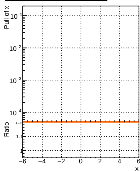
Legend: Blue line: DOM original Red line: DOM initialStepReso Black line: DOM initialStepReso Chi2Zero Orange line: DOM initialStepReso Grey line: DOM initialStepReso
