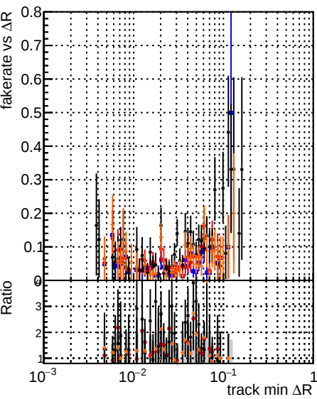
Fake rate vs \Delta R(\text{track, jet}) DQM original4 DQM testIMKFit initialStepReso DQM testIMKFit initialStepReso Chi2Zero
