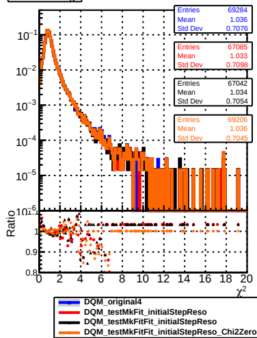
normalized \chi^2
