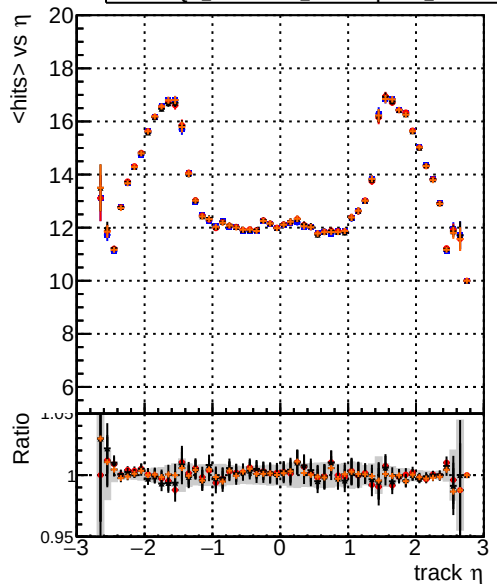
mean hits vs \eta Legend: DQM_original4 DQM_testMkFit_initialStepReso DQM_testMkFitFit_initialStepReso DQM_testMkFitFit_initialStepReso_Chi2Zero
