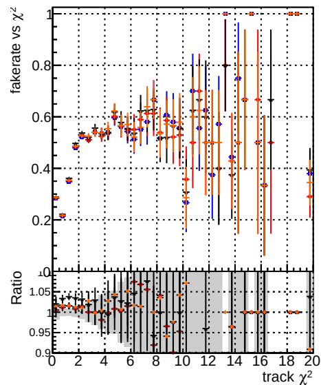
Fake rate vs. DQM test MKFit Fit Initial Step Res0 Chi2Zero
