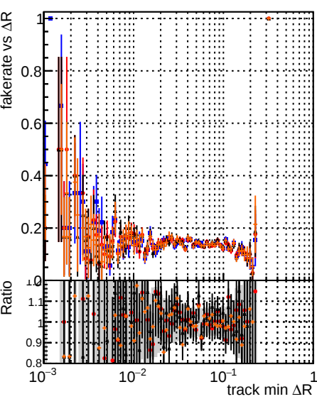
Fake rate vs \Delta R(\text{track, jet}) Duplicates Rate
