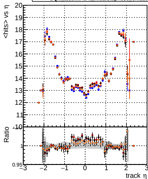
mean hits vs \eta Legend: — DQM_testMkFit_initialStepReso — DQM_testMkFitFit_initialStepReso — DQM_testMkFitFit_initialStepReso_Chi2Zero
