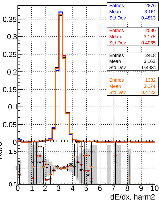
— DQM_original4 — DQM_testMkFit_initialStepReso — DQM_testMkFitFit_initialStepReso — DQM_testMkFitFit_initialStepReso_Chi2Zero
