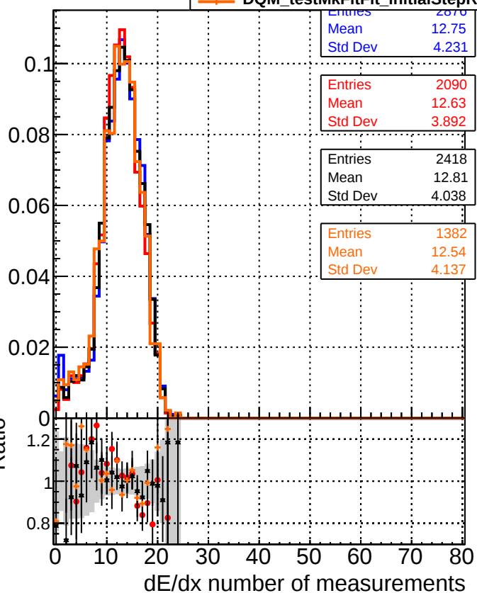
— DQM_original4 — DQM_testMkFit_initialStepReso — DQM_testMkFitFit_initialStepReso — DQM_testMkFitFit_initialStepReso_Chi2Zero
