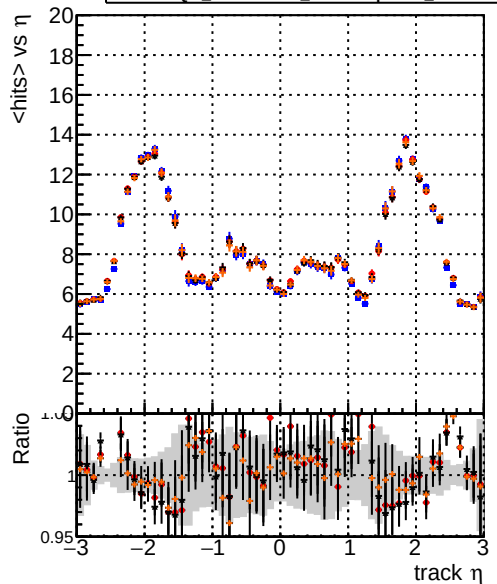
— DQM_original4 — DQM_testMkFit_initialStepReso — DQM_testMkFitFit_initialStepReso — DQM_testMkFitFit_initialStepReso_Chi2Zero mean hits
