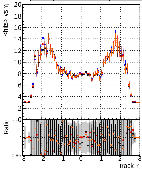
mean hit DQM_original4 DQM_testMkFitFit_initialStepReso DQM_testMkFitFit_initialStepReso_chi2Zero
