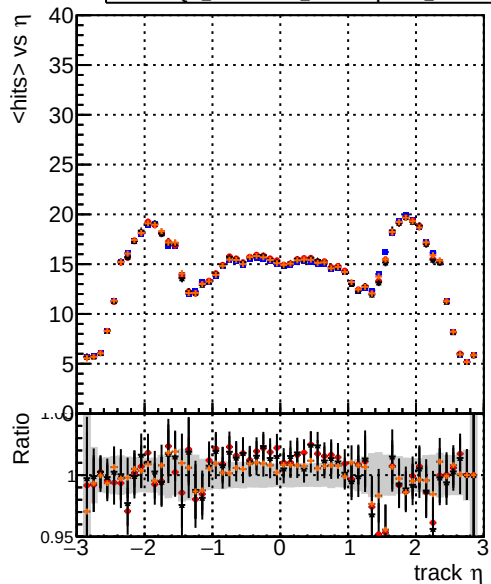
mean hits DQM_origMkFit4 DQM_testMkFitFit_initialStepReso DQM_testMkFitFit_initialStepReso DQM_testMkFitFit_initialStepReso_Chi2Zero
