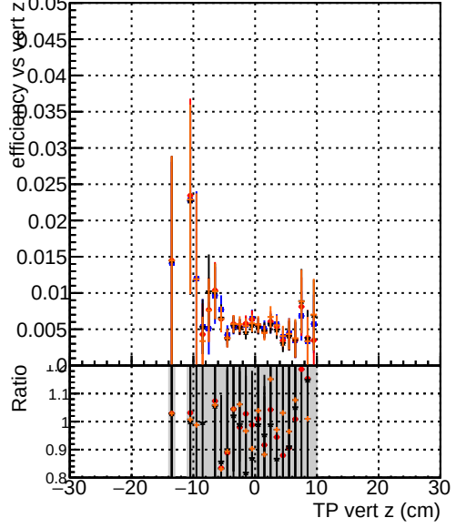
Efficiency vs TP vert z — DQM_original4 — DQM_testMkFit_fit_initialStepReso — DQM_testMkFitFit_initialStepReso — DQM_testMkFitFit_initialStepReso_chi2Zero
