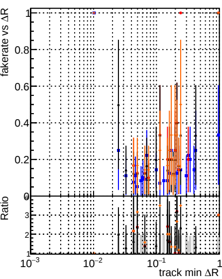
Fake rate vs \Delta R(\text{track, jet}) for DOM original, DOM test, DOM MC Fit initialStepReso, and DOM test MC Fit initialStepReso Chi2Zero
