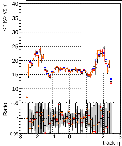
mean hits DQM_original4 DQM_testMkFit_initialStepReso DQM_testMkFitFit_initialStepReso DQM_testMkFitFit_initialStepReso_chi2Zero
