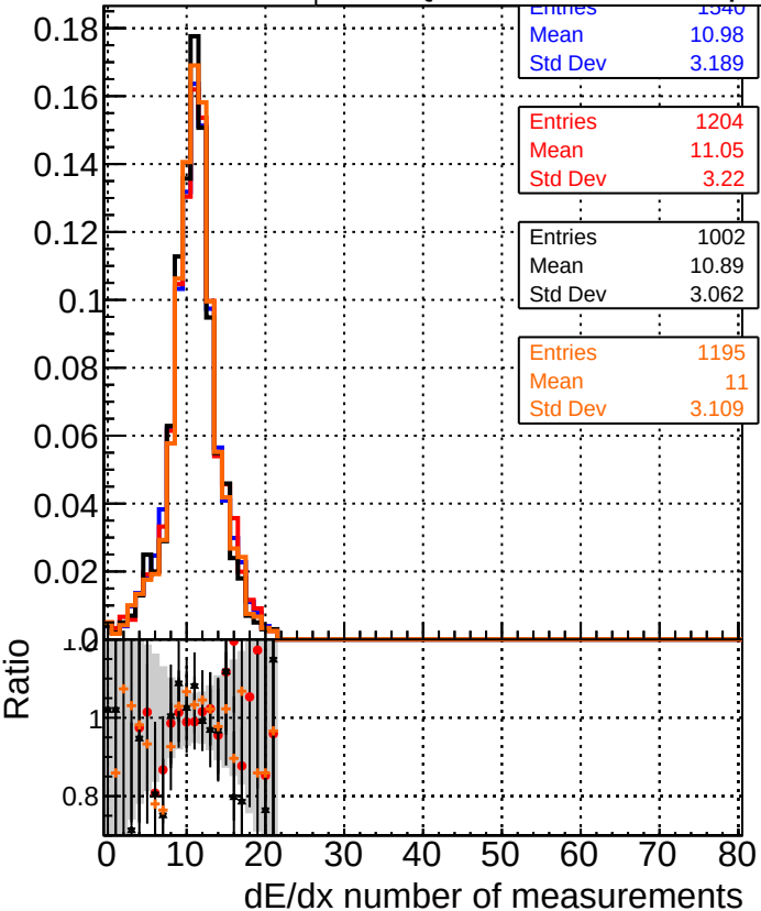
—●— DQM_original4 —●— DQM_testMkFit_initialStepReso —●— DQM_testMkFitFit_initialStepReso —●— DQM_testMkFitFit_initialStepReso_Chi2Zero
