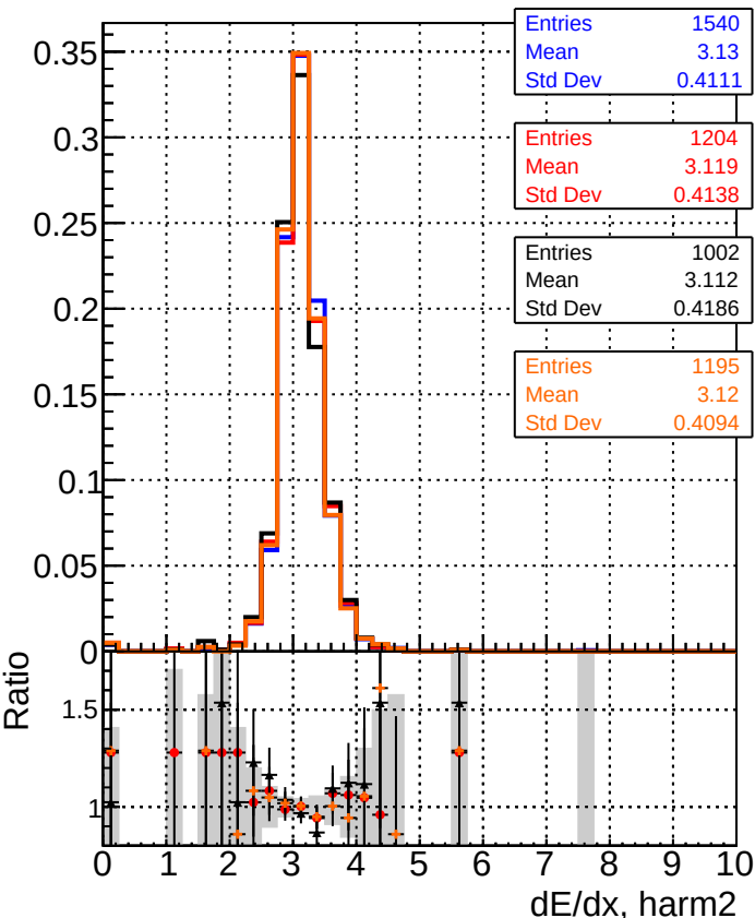
—●— DQM_original4 —●— DQM_testMkFit_initialStepReso —●— DQM_testMkFitFit_initialStepReso —●— DQM_testMkFitFit_initialStepReso_Chi2Zero
