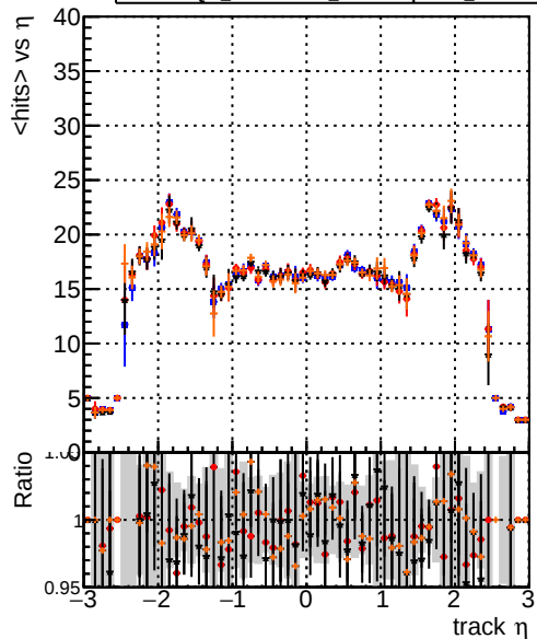
mean hits vs \eta DQM_original4 DQM_testMkFit_initialStepReso DQM_testMkFitFit_initialStepReso DQM_testMkFitFit_initialStepReso_Chi2Zero
