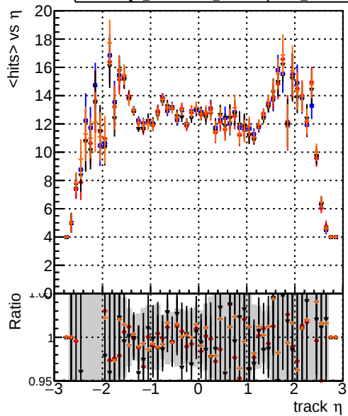
mean hits DQM_original4 DQM_testMkFit_fit_initialStepReso DQM_testMkFit_fit_initialStepReso DQM_testMkFit_fit_initialStepReso_chi2Zero
