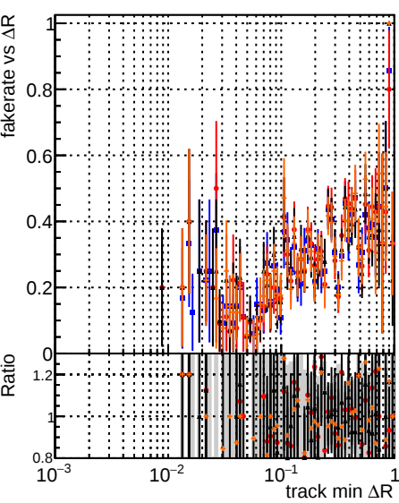
Fake rate vs \Delta R(\text{track, jet}) DOM original DOM test DOM fit initialStepReso DOM fit initialStepReso Chi2Zero
