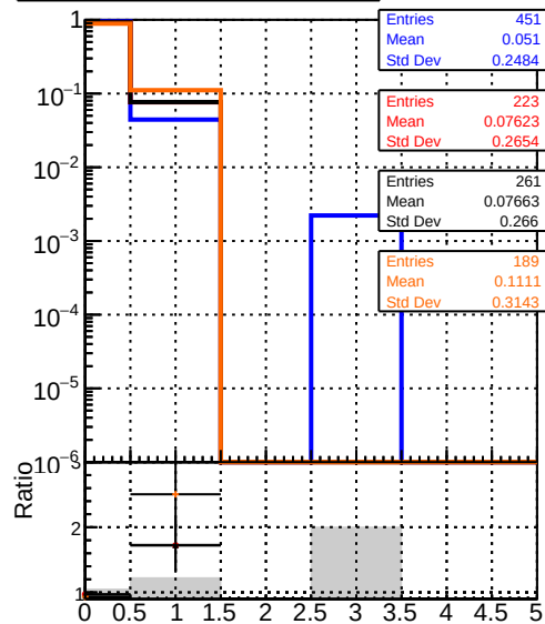
mean hit — DQM_original4 — DQM_testMkFit_fit_initialStepReso — DQM_testMkFitFit_initialStepReso — DQM_testMkFitFit_initialStepReso_chi2Zero
