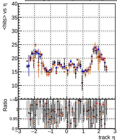
mean hit — DQM_original4 — DQM_testMkFit_fit_initialStepReso — DQM_testMkFitFit_initialStepReso — DQM_testMkFitFit_initialStepReso_chi2Zero
