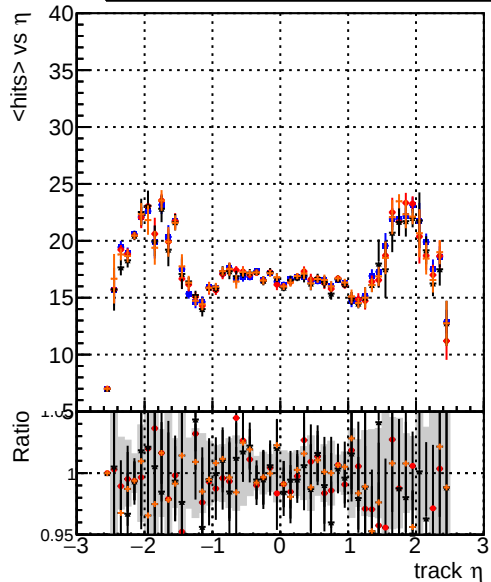
mean hit — DQM_original4 — DQM_testMkFit_initialStepReso — DQM_testMkFitFit_initialStepReso — DQM_testMkFitFit_initialStepReso_Chi2Zero
