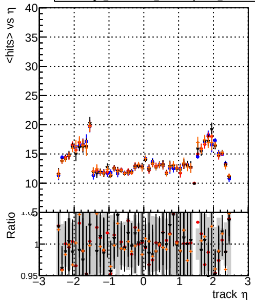
DQM_testMkFitFit_initialStepReso DQM_testMkFitFit_initialStepReso DQM_testMkFitFit_initialStepReso DQM_testMkFitFit_initialStepReso_Chi2Zero mean hits
