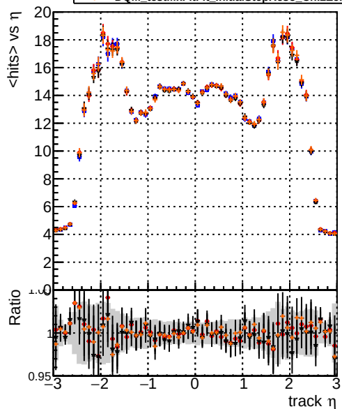
mean hit Legend: - DQM_original4 (blue line with circles) - DQM_testMkFit_initialStepReso (red line with circles) - DQM_testMkFitFit_initialStepReso (black line with circles) - DQM_testMkFitFit_initialStepReso_Chi2Zero (orange line with circles)
