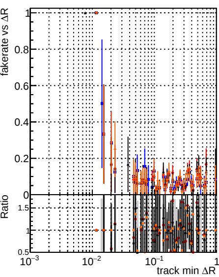
Fake rate vs \Delta R(\text{track, jet}) DOM original DOM test DOM fit DOM fit initialStepReso DOM fit initialStepReso Chi2Zero
