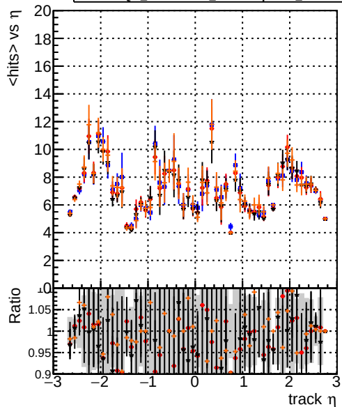
mean hit Legend: DQM_original4 (blue line) DQM_testMkFit_initialStepReso (red line with dots) DQM_testMkFitFit_initialStepReso (black line with dots) DQM_testMkFitFit_initialStepReso_chi2Zero (orange line with dots)
