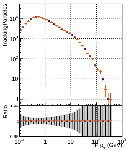
● DQM_original4 ● DQM_testMkFit_initialStepReso ● DQM_testMkFitFit_initialStepReso ● DQM_testMkFitFit_initialStepReso_ChizZero
