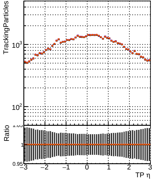
● DQM_original4 ● DQM_testMkFit_initialStepReso ● DQM_testMkFitFit_initialStepReso ● DQM_testMkFitFit_initialStepReso_ChizZero
