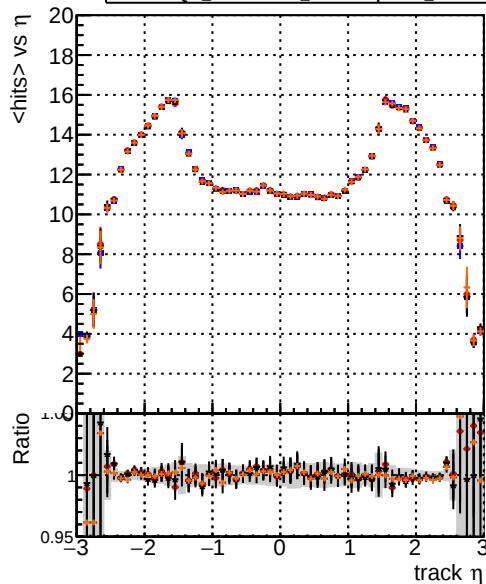
mean hit DQM_testMkFit_initialStepReso DQM_testMkFitFit_initialStepReso DQM_testMkFitFit_initialStepReso_chi2Zero
