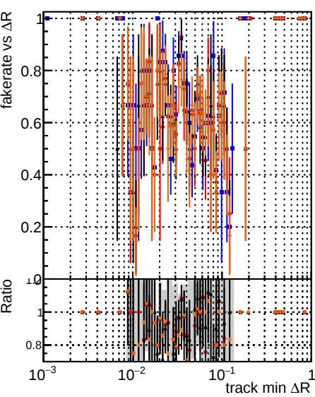
Fake rate vs \Delta R(\text{track, jet}) DOM original4 DOM testIMKFit initialStepReso DOM testIMKFit initialStepReso DOM testIMKFit initialStepReso Chi2Zero
