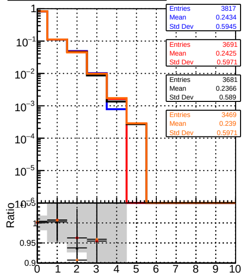
DQM_original4 DQM_testMkFit_initialStepReso DQM_testMkFitFit_initialStepReso DQM_testMkFitFit_initialStepReso_chi2Zero
