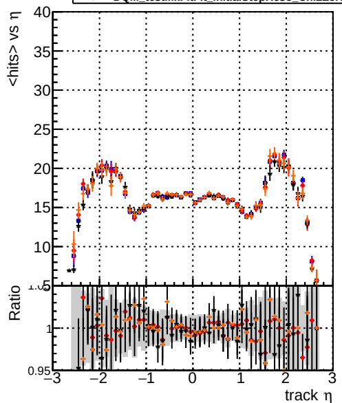
DQM_original4 DQM_testMkFit_initialStepReso DQM_testMkFitFit_initialStepReso DQM_testMkFitFit_initialStepReso_chi2Zero
