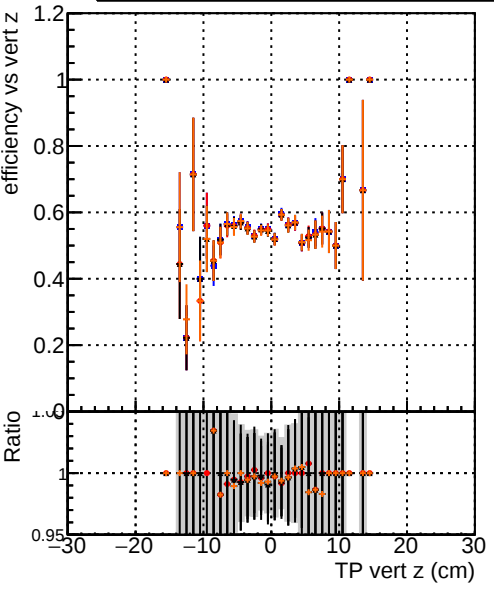
Efficiency vs vertpos DQM_original4 DQM_testMkFit_initialStepReso DQM_testMkFitFit_initialStepReso DQM_testMkFitFit_initialStepReso_Chi2Zero
