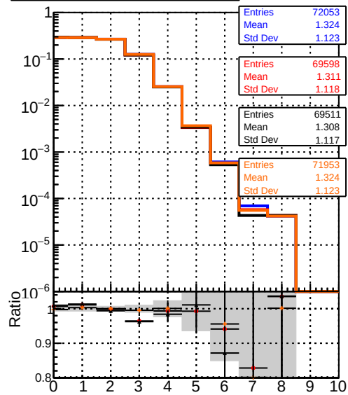
DQM_testMkFitFit_initialStepReso DQM_testMkFitFit_initialStepReso DQM_testMkFitFit_initialStepReso_chi2Zero mean hits
