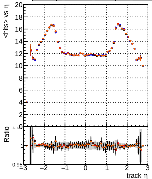
DQM_testMkFitFit_initialStepReso DQM_testMkFitFit_initialStepReso DQM_testMkFitFit_initialStepReso_chi2Zero mean hits
