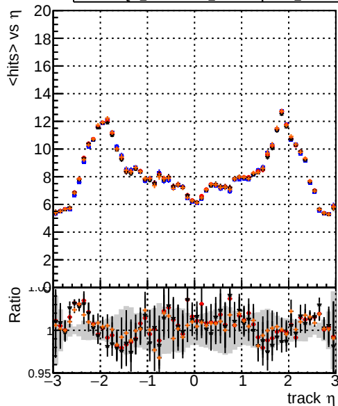
— DQM_original4 — DQM_testMkFit_initialStepReso — DQM_testMkFitFit_initialStepReso — DQM_testMkFitFit_initialStepReso_Chi2Zero mean hits
