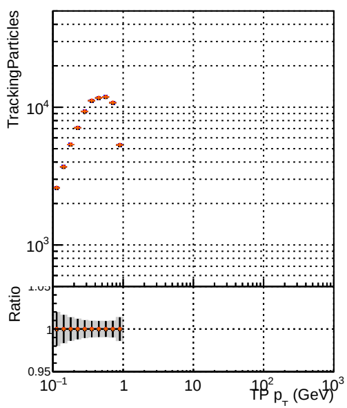
● DQM_original4 ● DQM_testMkFitFit_initialStepReso ● DQM_testMkFitFit_initialStepReso ● DQM_testMkFitFit_initialStepReso_wRejection5
