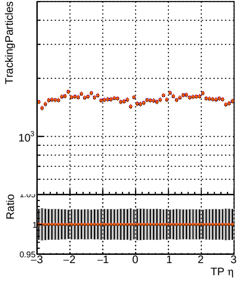
● DQM_original4 ● DQM_testMkFitFit_initialStepReso ● DQM_testMkFitFit_initialStepReso ● DQM_testMkFitFit_initialStepReso_wRejection5
