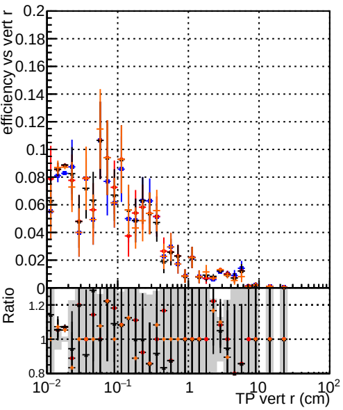
Efficiency vs TP vert r (cm) DQM_original4 DQM_testMkFit_initialStepReso DQM_testMkFitFit_initialStepReso DQM_testMkFitFit_initialStepReso_wRejection5
