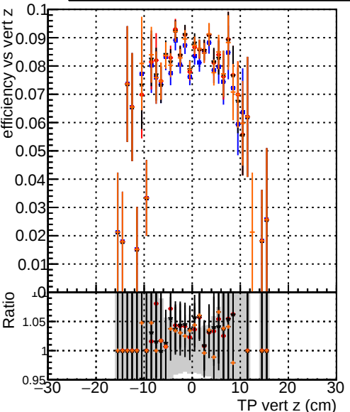
Efficiency vs vertpos Legend: DQM_original4 DQM_testMkFit_initialStepReso DQM_testMkFitFit_initialStepReso DQM_testMkFitFit_initialStepReso_wRejection5
