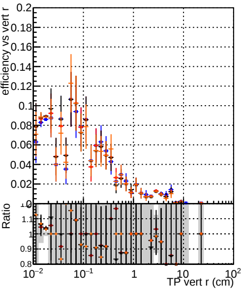
Efficiency vs vertpos Legend: DQM_original4 DQM_testMkFit_initialStepReso DQM_testMkFitFit_initialStepReso DQM_testMkFitFit_initialStepReso_wRejection5
