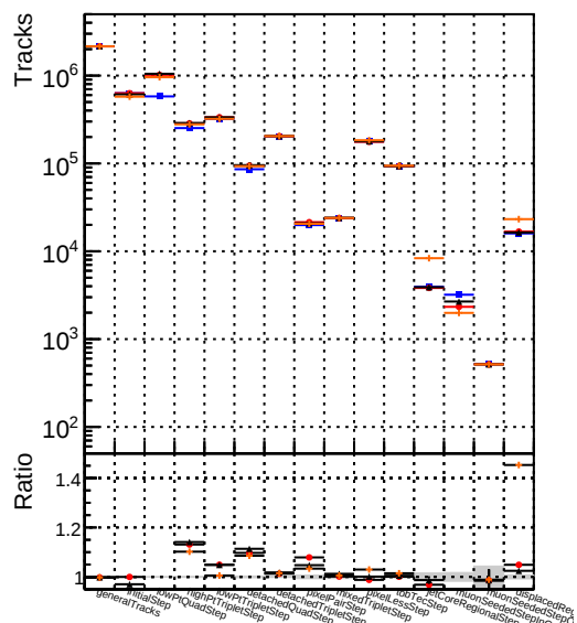
Number of tracks vs collection DQM_original4 DQM_testMkFit_initialStepReso DQM_testMkFitFit_initialStepReso DQM_testMkFitFit_initialStepReso_wRejection5
