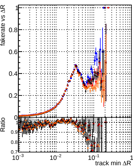
Fake rate vs \Delta R (track, jet) for different methods: DOM original, DOM fit, DOM fit initialStepReso, DOM fit initialStepReso wRejection5
