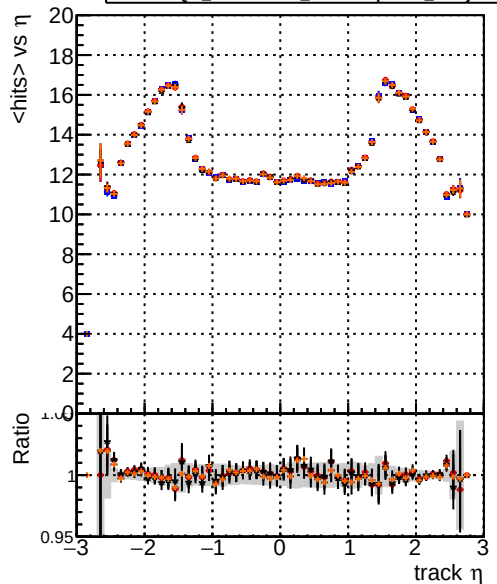
DQM_testMkFitFit_initialStepReso DQM_testMkFitFit_initialStepReso DQM_testMkFitFit_initialStepReso_wRejection5 mean hit
