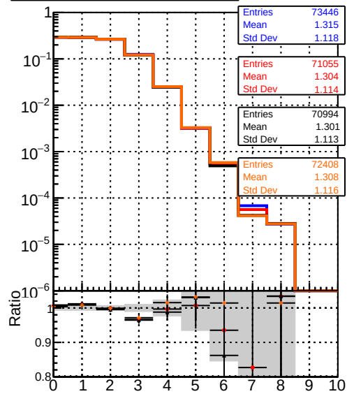
DQM_testMkFitFit_initialStepReso DQM_testMkFitFit_initialStepReso DQM_testMkFitFit_initialStepReso_wRejection5 mean hit
