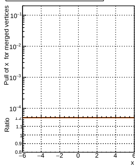
RecoAllAssoc2GenMatchedMerged_PullX
