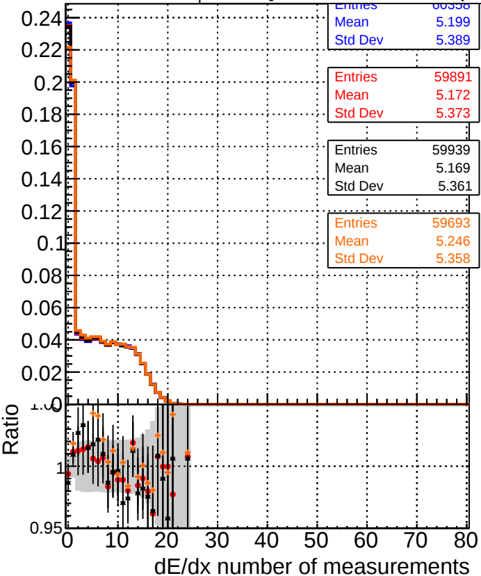
—●— DQM_original4 —●— DQM_testMkFit_initialStepReso —●— DQM_testMkFitFit_initialStepReso —●— DQM_testMkFitFit_initialStepReso_wRejection5
