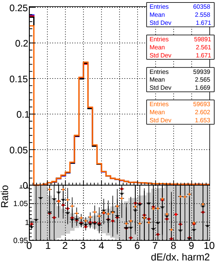
—●— DQM_original4 —●— DQM_testMkFit_initialStepReso —●— DQM_testMkFitFit_initialStepReso —●— DQM_testMkFitFit_initialStepReso_wRejection5
