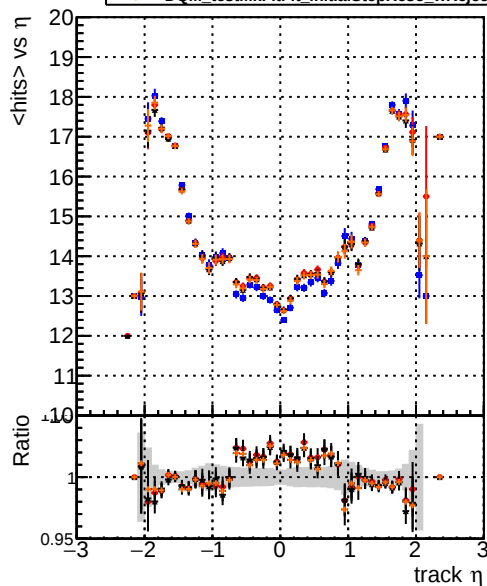
mean hit DQM_testMkFit_initialStepReso DQM_testMkFitFit_initialStepReso DQM_testMkFitFit_initialStepReso_wRejection5
