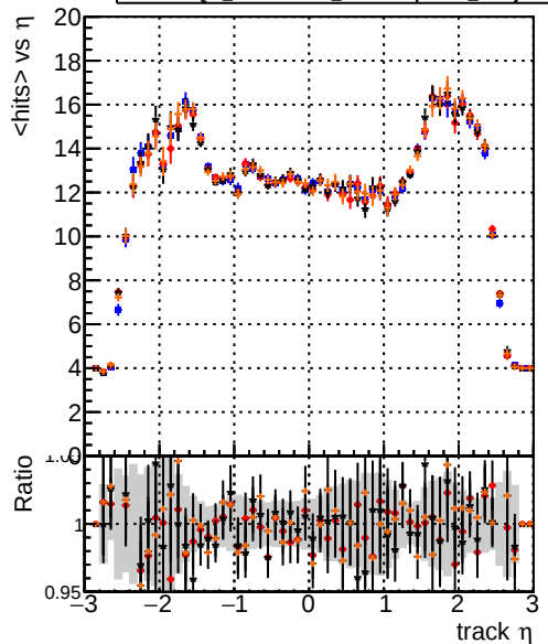
DQM_testMkFitFit_initialStepReso DQM_testMkFitFit_initialStepReso DQM_testMkFitFit_initialStepReso DQM_testMkFitFit_initialStepReso_wRejection5 mean hit
