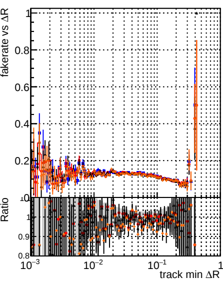
Fake rate vs \Delta R (track, jet) Duplicates rate vs \Delta R (track, jet) Pileup rate vs \Delta R (track, jet) wRejection5
